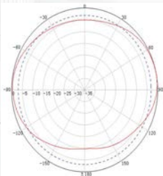
H-plane:Gain11.2dBi 1/2WL.spacing from tower
