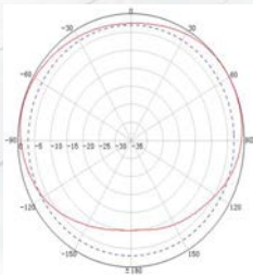
H-plane:Gain10.6dBi 3/8WL.spacing from tower
