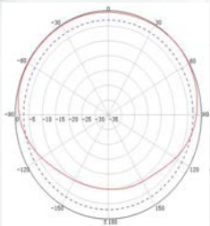
H-plane:Gain11.2 dBi 1/4WL.spacing from tower
