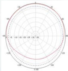
H-plane: Gain 11.2 dBi 1/4WL spacing from tower
