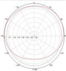
H-plane: Gain 10.6 dBi 3/8WL spacing from tower
