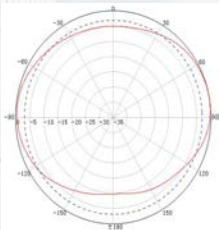
H-plane: Gain 11.2 dBi 1/2WL spacing from tower
